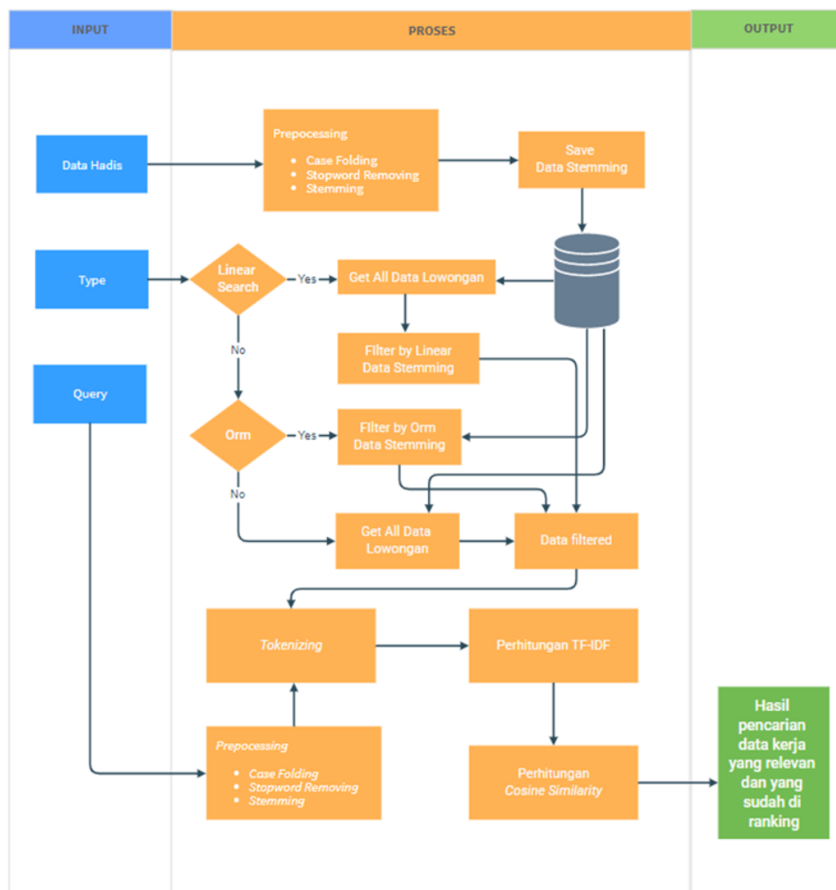
Figure 3. System flowchart
