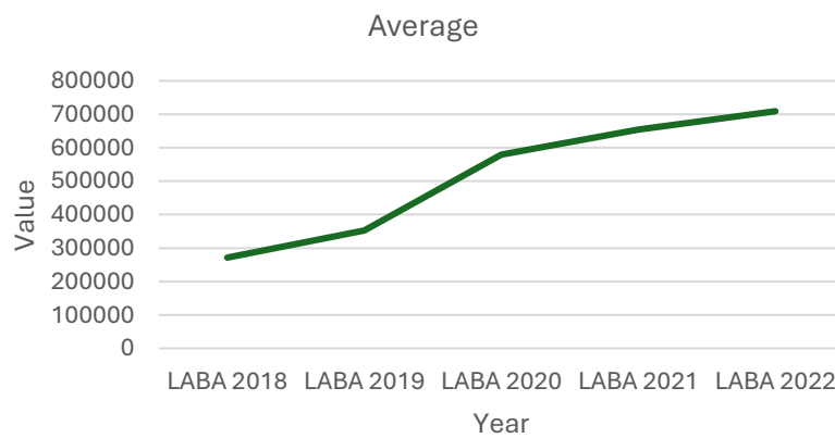
Figure 10. Average profit cluster 1
