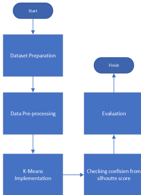
Figure 3. Implementation k-means
