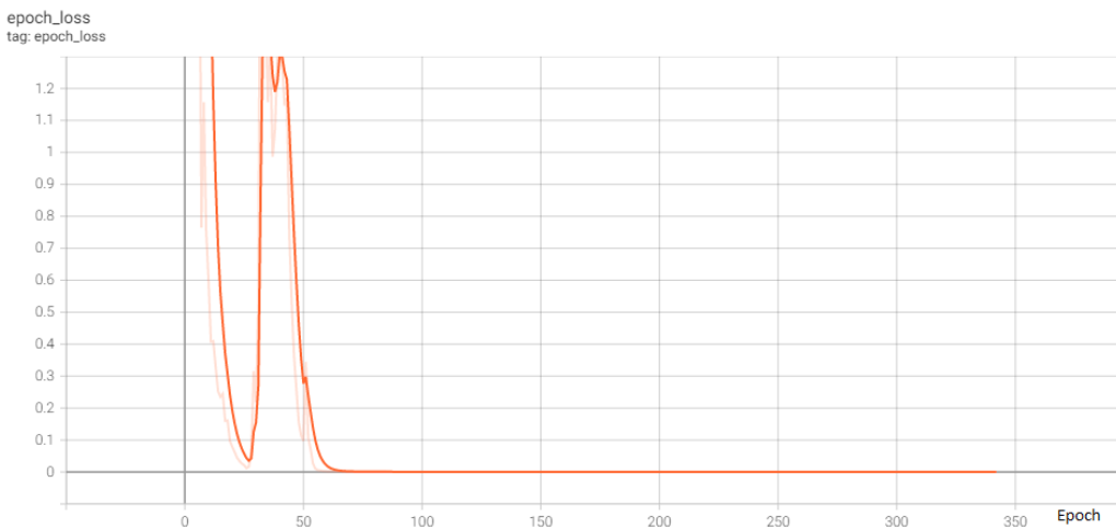
Figure 4. Epoch loss
