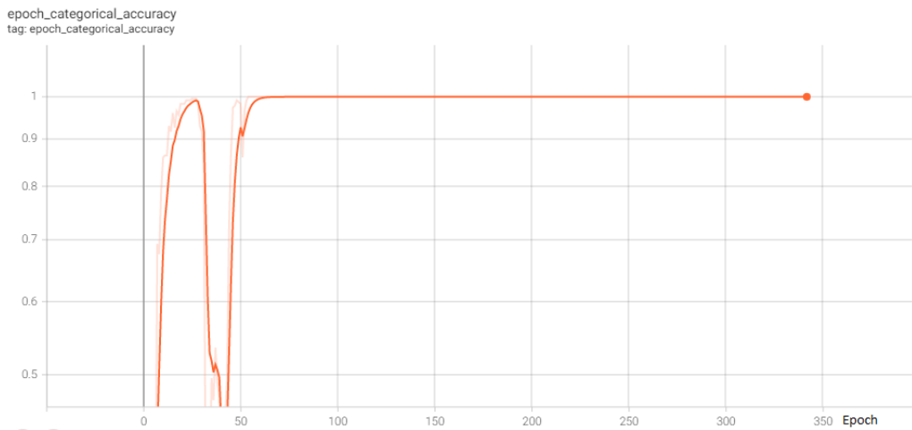
Figure 3. Categorical accuracy
